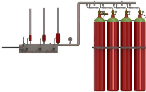
Figure 12. Selector Valve Setup
